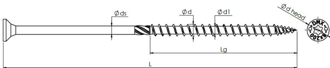
Figure 1: Screw, type CS
